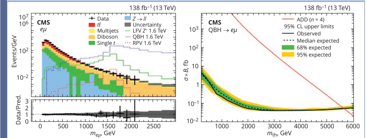
Fig. 8. Invariant mass distribution for the e\mu channel (left); 95% CL upper limits on the product of the cross section and the branching fraction for quantum black hole production in an ADD model with n = 4 extra dimensions, in the e\mu channel (right)
