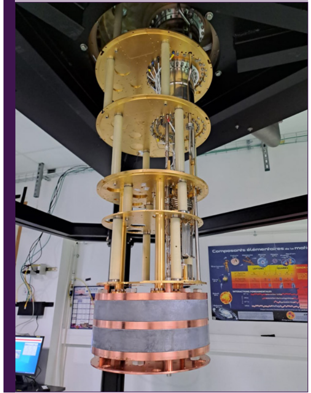
^3\text{He} - ^4\text{He} Ricochet dilution cryostat during the final commissioning phase at IP2I (Lyon) before its delivery to the ILL site
