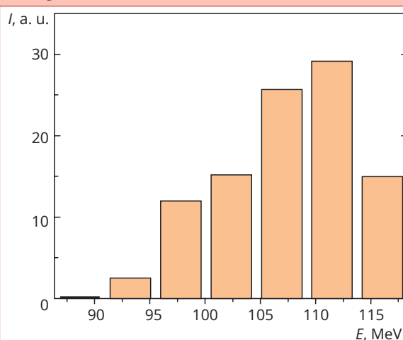
Fig. 5. Energy spectrum of accelerated electrons. By adjusting the frequency of the master oscillator, the natural frequencies of the SLED systems, the phase of the second accelerating section and the startup delay of the electron beam in relation to the microwave “phase reversal”, the average beam energy at the output of the accelerator can be brought to a value of more than 100 MeV
