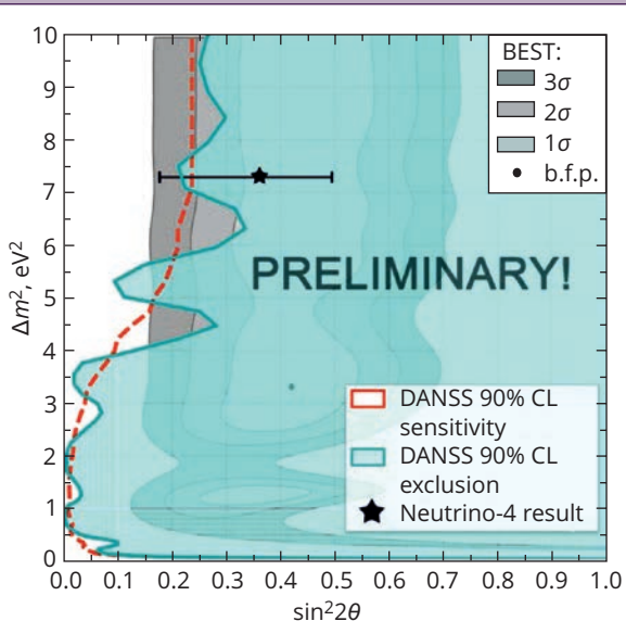
Fig. 2. Exclusion area at 90% CL in parameter space for sterile neutrino calculated with the raster scan method (blue area) and the sensitivity area (red dotted line)
