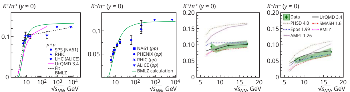
Fig. 9. Comparison of experimental data on the yield of kaons and pions in pp and BeBe collisions with calculations of the JINR group (BMLZ), as well as other models (Epos 1.99, UrQMD 3.4, PHSD 4.0, AMPT 1.26, SMASH 1.6)
