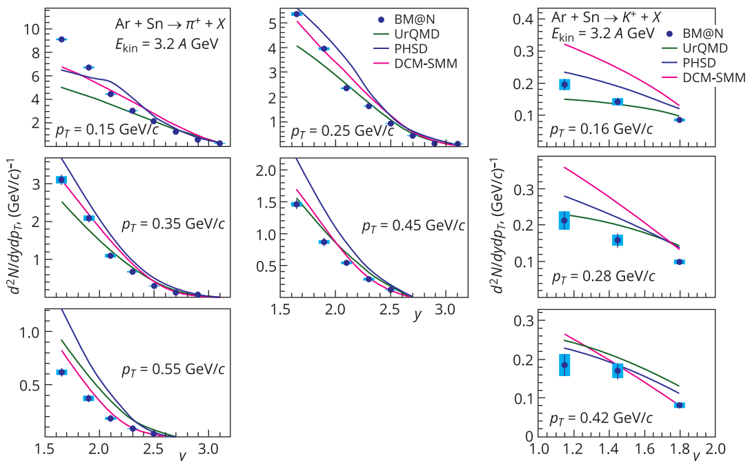
Fig. 3. The yields of \pi^+ and K^+ mesons depending on the rapidity in different intervals of the transverse momentum. The data are compared with predictions of the UrQMD, DCM-SMM and PHSD models of nucleus-nucleus interactions
