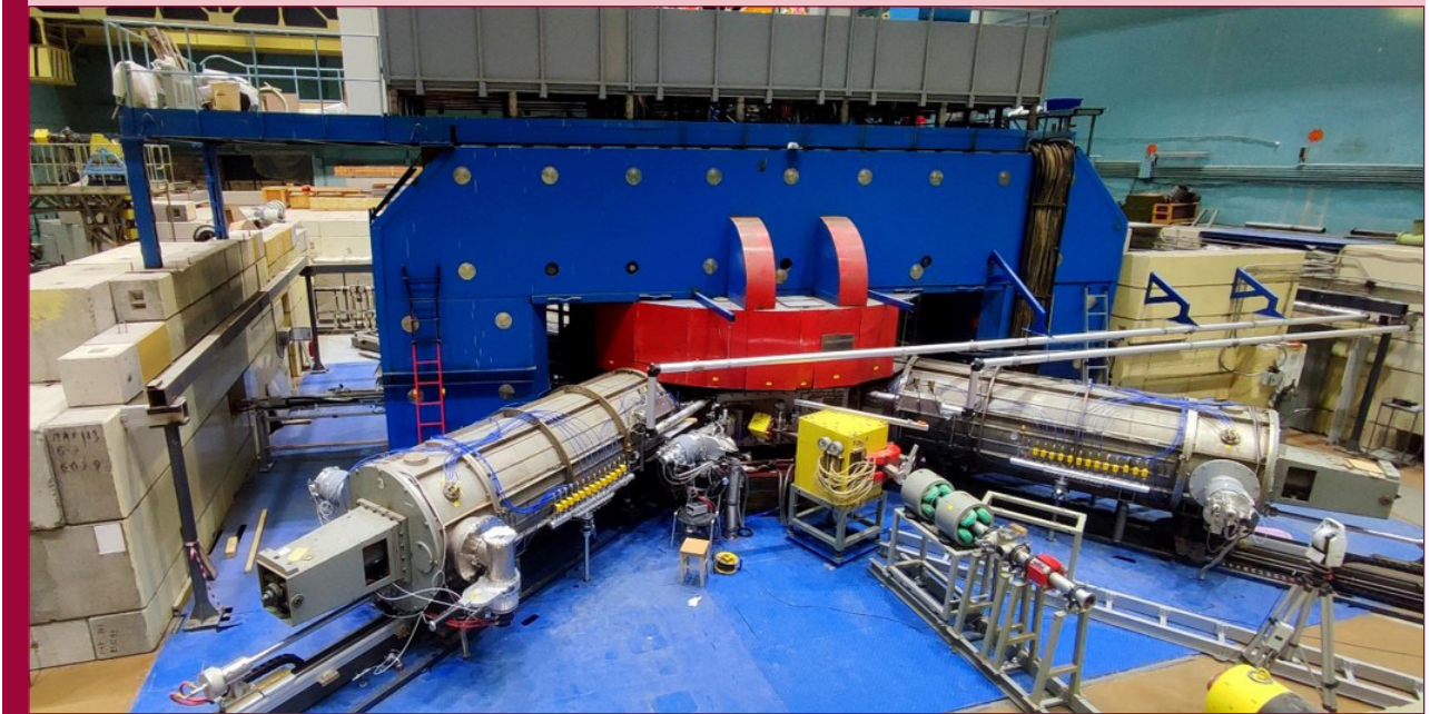
U-400M accelerator
