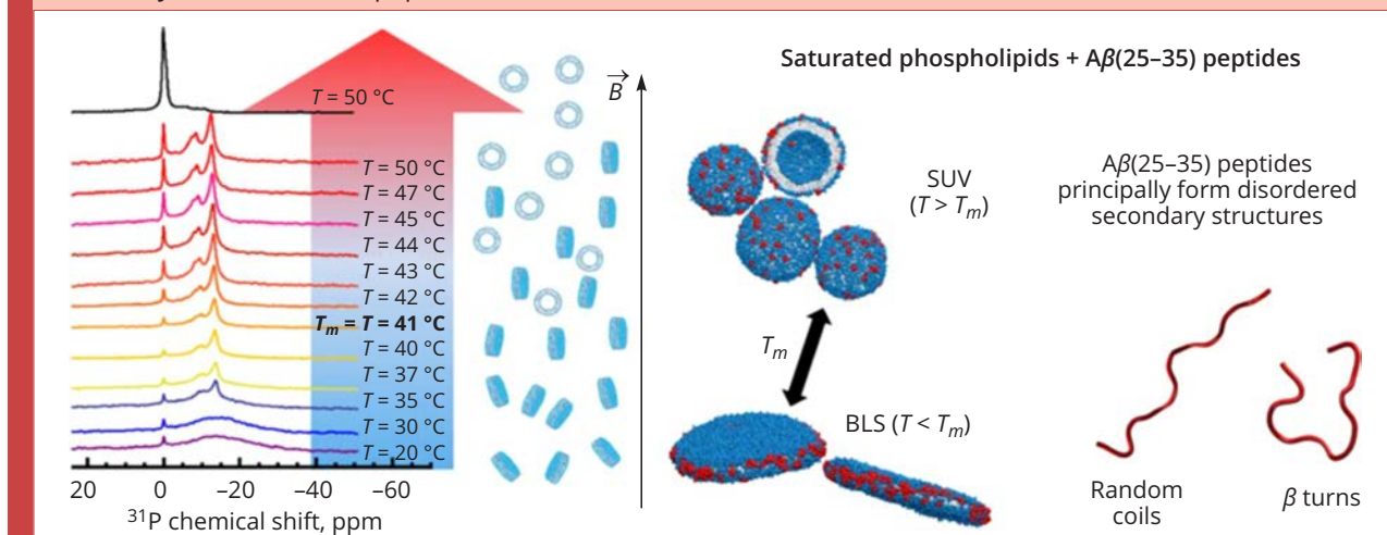
Fig. 3. ^{31}\text{P} NMR spectra of the lipid-peptide system DPPC + A \beta (25–35) at different temperatures, as well as visualization of the structure of the observed BLSs obtained using molecular dynamics simulations, and the secondary structure of the peptides
